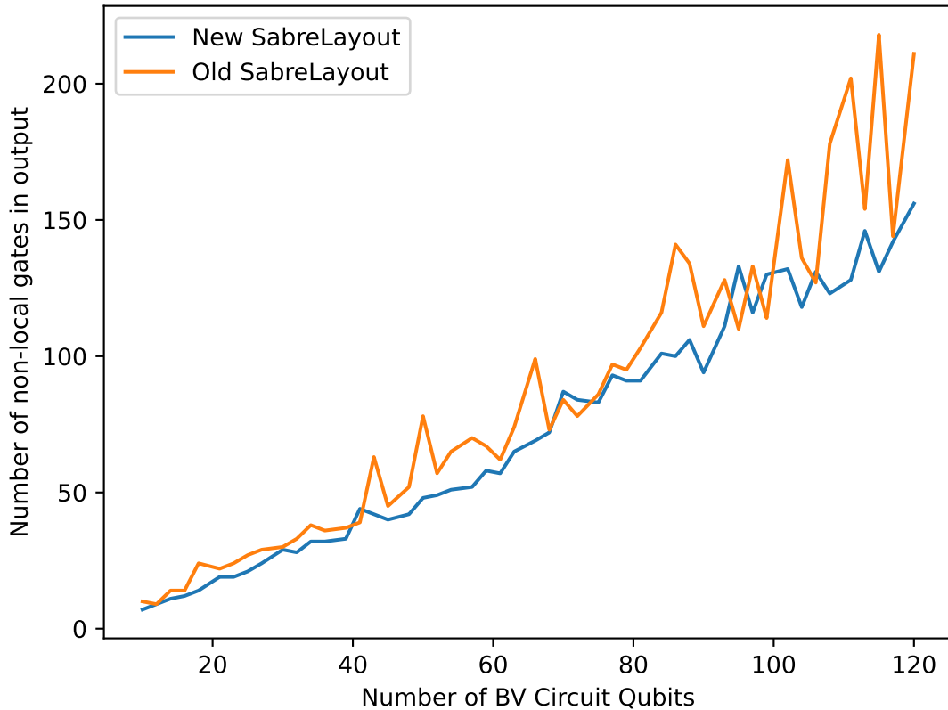
Number of non-local gates after SabreLayout and SabreSwap
